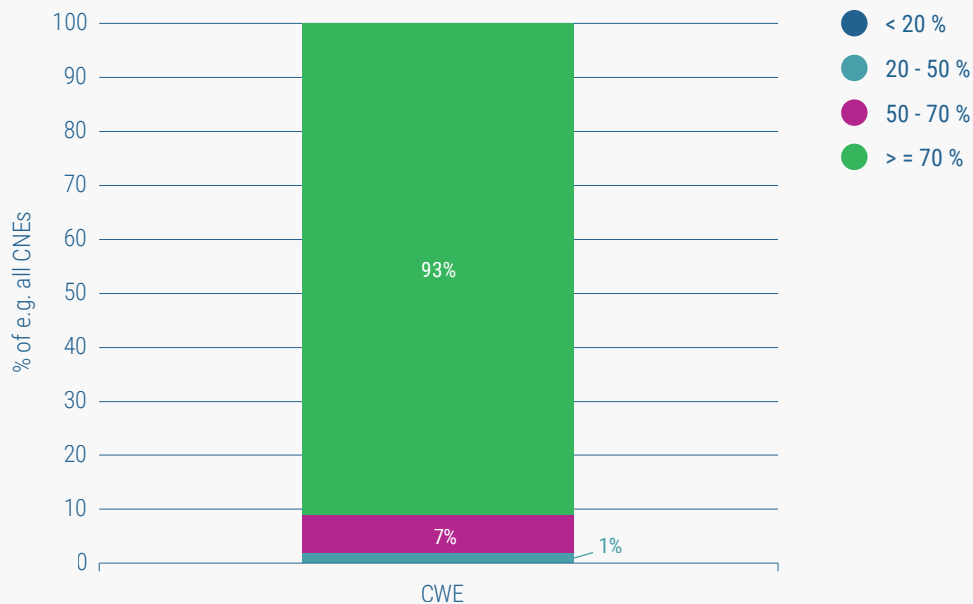
Relative cross-zonal trading margin of TransnetBW for CWE with a minimum capacity of 11.5%
