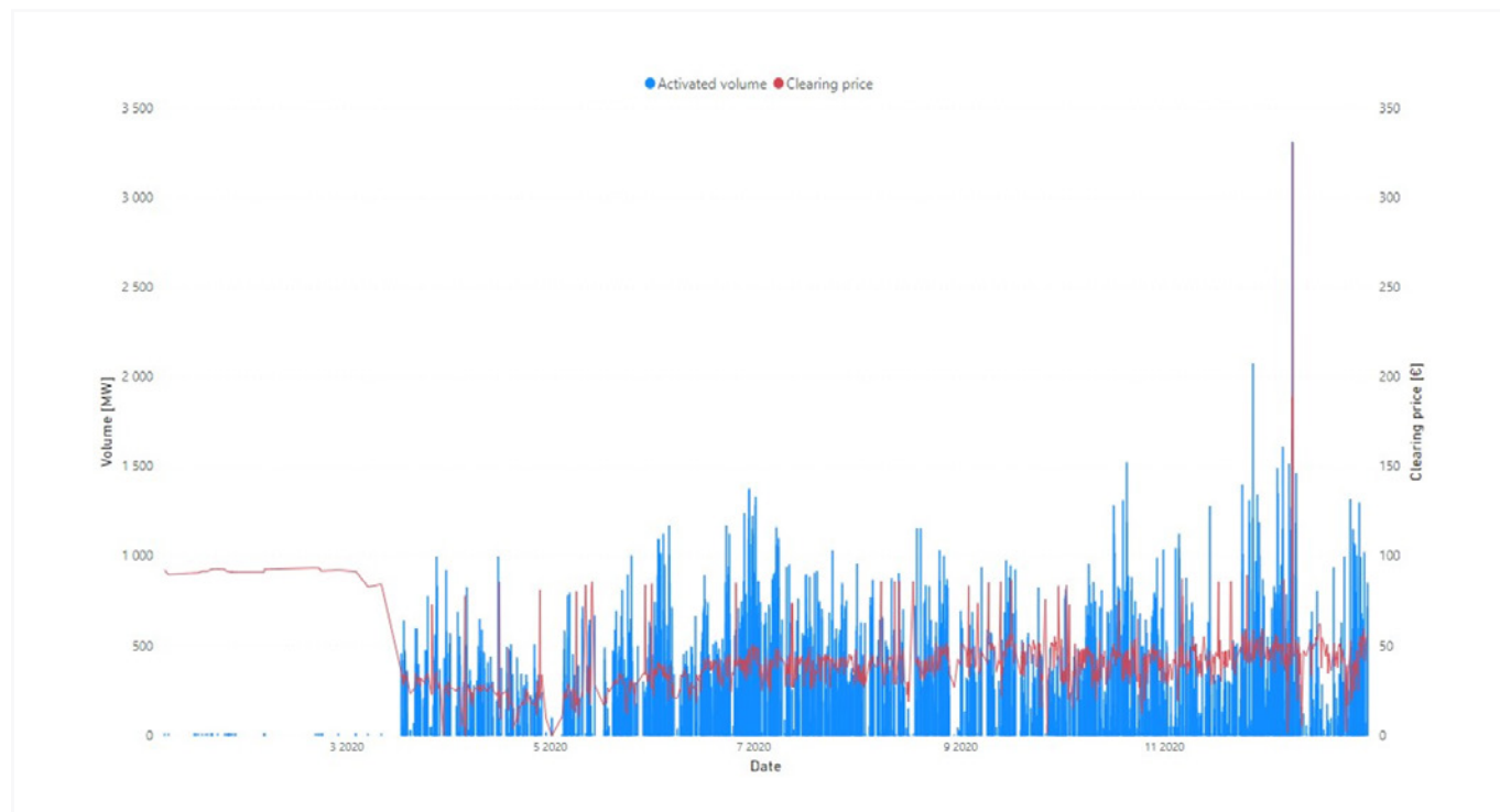
Figure 33 – Volumes and clearing price of activated upward standard balancing RR bids
