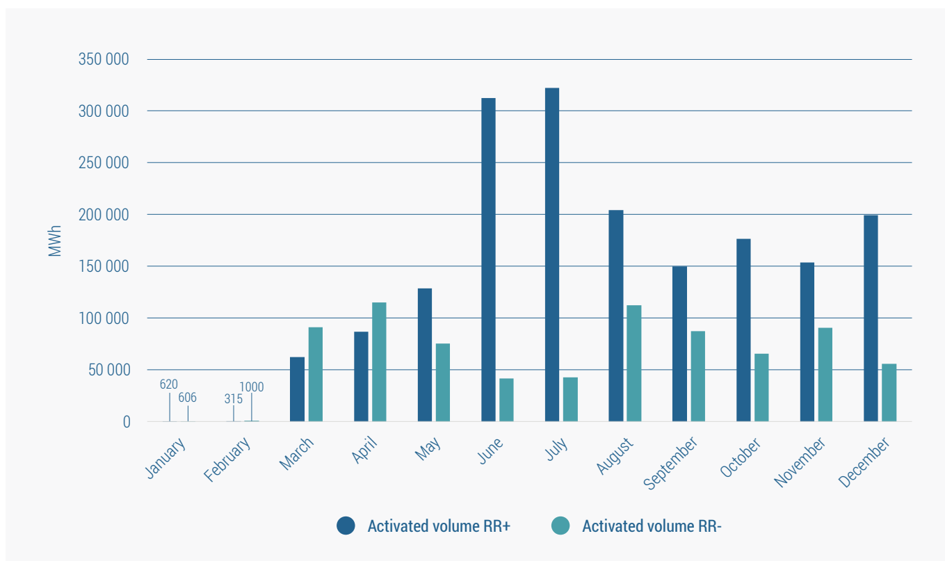
Figure 27 – Monthly activated volume (in MWh) on the RR platform in 2020
