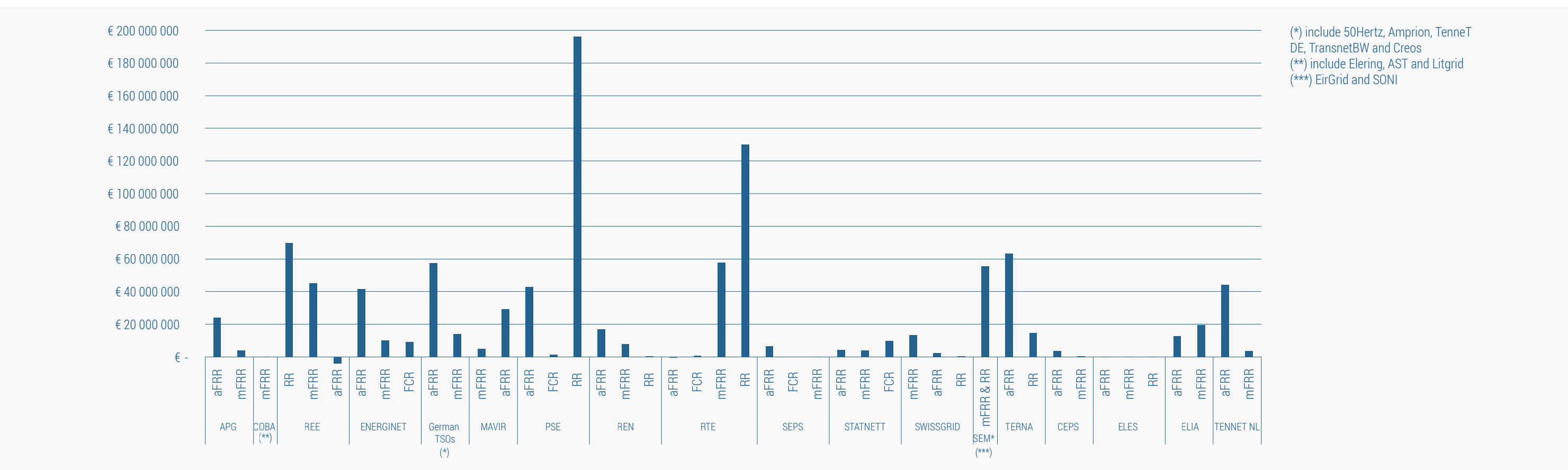
Figure 66 – Total yearly cost of activation of balancing energy from contracted (Source: Data submitted by each TSO)
