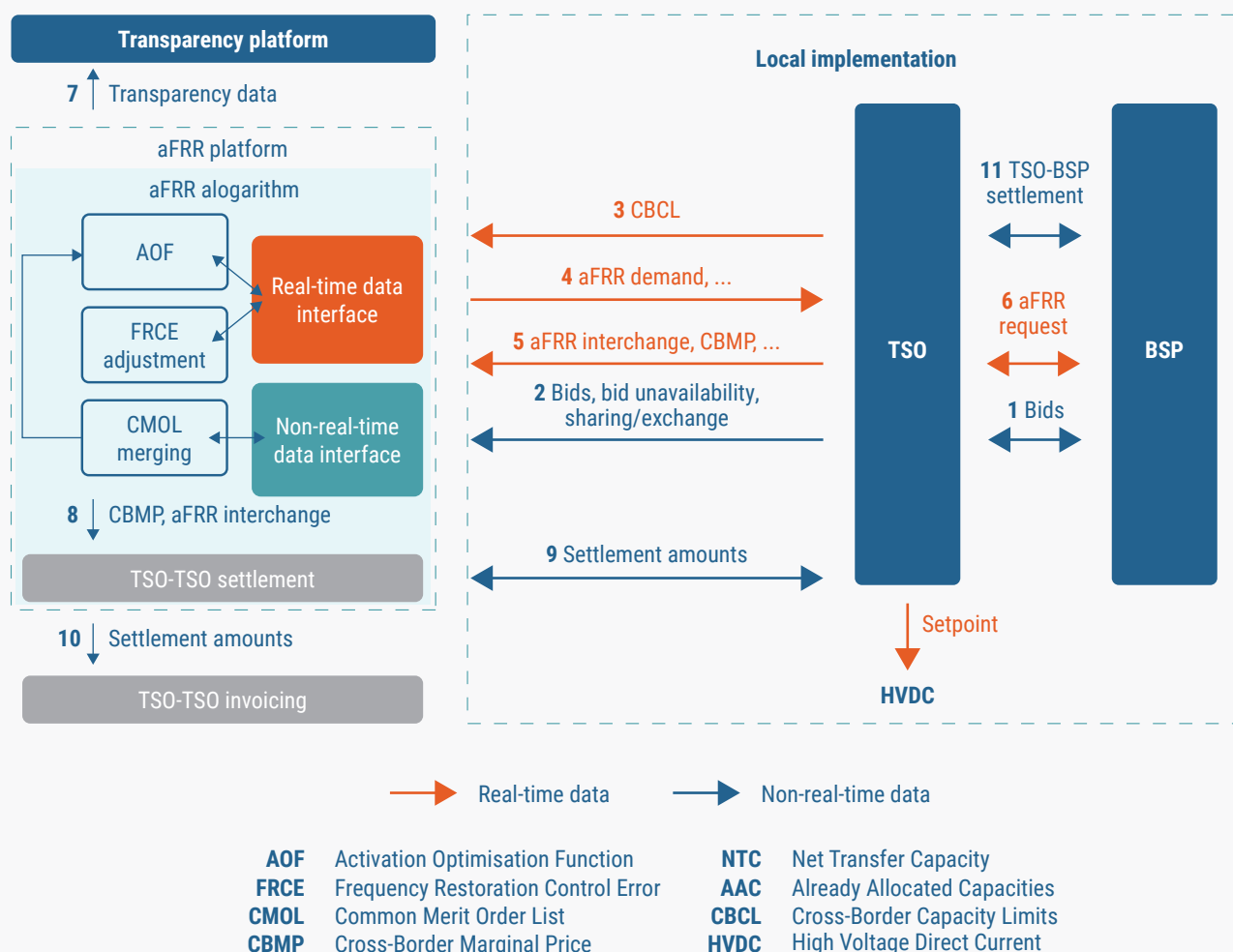
Figure 43 – PICASSO High-Level Design (as of February 2021)
