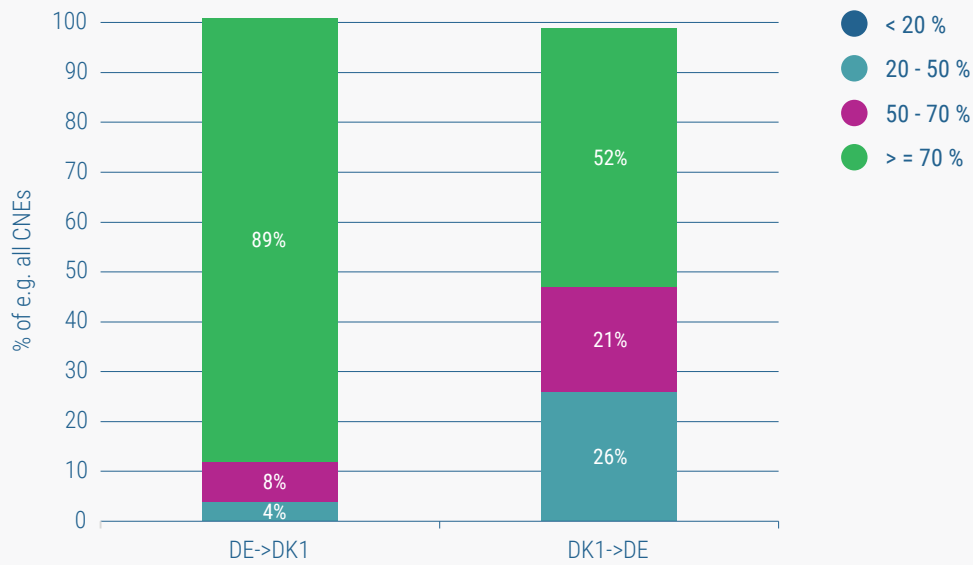
Relative cross-zonal trading margin of TenneT Germany DE→DK1 and DK1→DE with a minimum NTC of 428 MW
